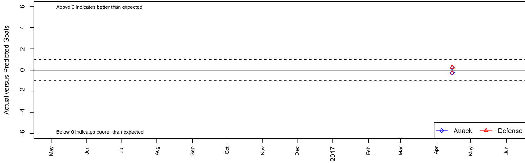
BYSL Fusion B99 Dots are actual minus expected GF (blue circles) and GA (red triangles). Blue line is smoothed change in attack strength. Red is smoothed change in defense strength.
